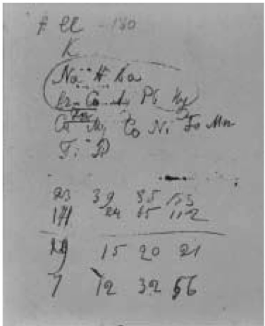
Mendeleev's first sketch of the periodic table of the elements Photograph by Nina Canell and Robin Watkins
